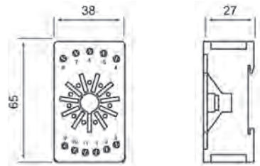
Base (Rail DIN)
