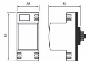
Base (Rail DIN)
